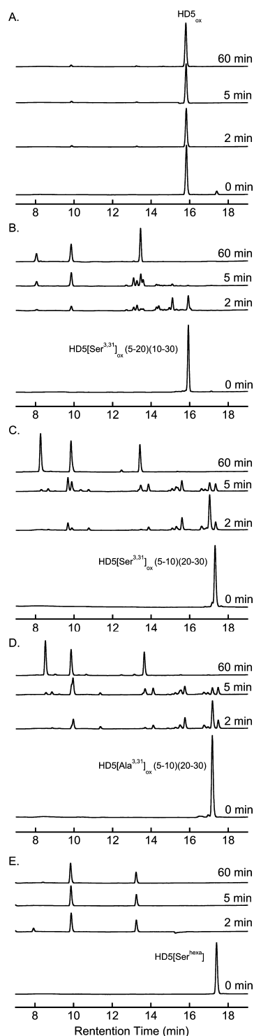
Figure 7. Analytical HPLC traces (220 nm) for trypsin susceptibility assays: (A) HD 5ox , (B) HD5[Ser 3,31 ] ox (5-20)(10-30), (C) HD5[Ser 3,31 ] ox (5-10)(20-30), (D) HD5[Ala 3,31 ] ox (5-10)(20-30), and (E) HD5[Ser hexa ].
