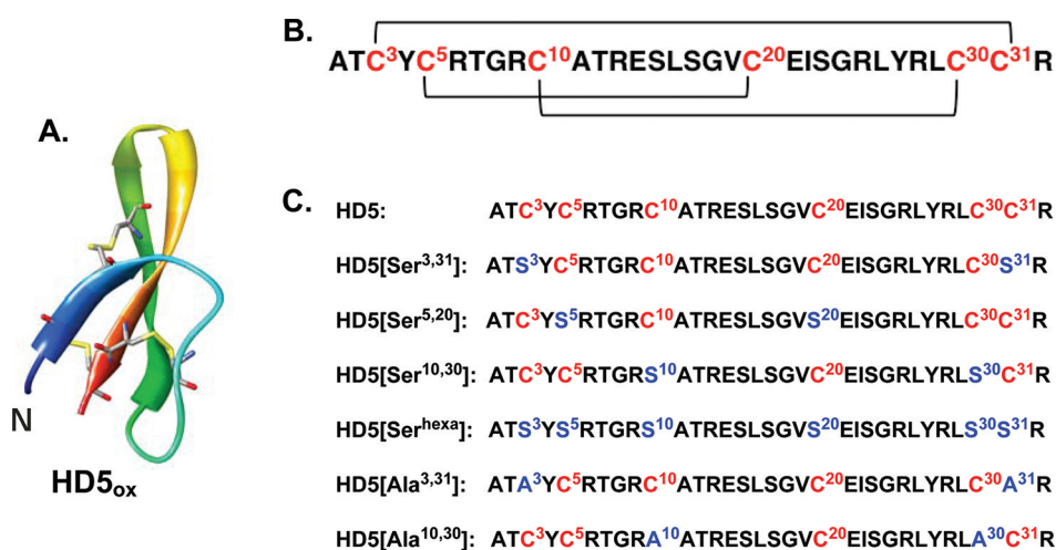
Figure 1. (A) X-ray crystal structure of HD5 ox (PDB 1ZMP, ref 38). The N-terminus is labeled in blue and the C-terminus is labeled in red. (B) Illustration of the Cys 3 -Cys 31 , Cys 5 -Cys 20 , and Cys 10 -Cys 30 disulfide linkages in native HD5 ox . (C) Nomenclature employed and amino acid sequences for the peptides studied in this work. Cys residues are depicted in red and the Ser/Ala mutations in blue.
