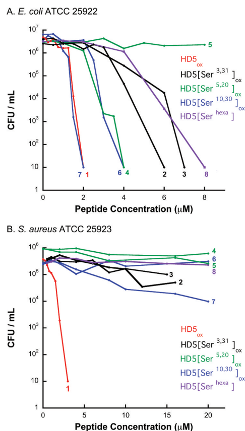
Figure 5. Antibacterial activity assays with the HD5 ox mutant family (CFU method). 1, HD5 ox ; 2, HD5[Ser 3,31 ] ox (5-30)(10-20); 3, HD5[Ser 3,31 ] ox (5-10)(20-30); 4, HD5[Ser 5,20 ] ox (3-31)(10-30); 5, HD5[Ser 5,20 ] ox (3-30)(10-31); 6, HD5[Ser 10,30 ] ox (3-31)(5-20); 7, HD5[Ser 10,30 ] ox (3-20)(5-31). (A) Activity of HD5 ox and the Ser mutants against E. coli ATCC 25922. (B) Activity of HD5 ox and the Ser mutants against S. aureus ATCC 25923. In both instances a CFU of 10 indicates no colony formation. The data represent the averages of three independent trials, and the error bars are omitted for clarity. Plots including error bars are provided as Supporting Information.
