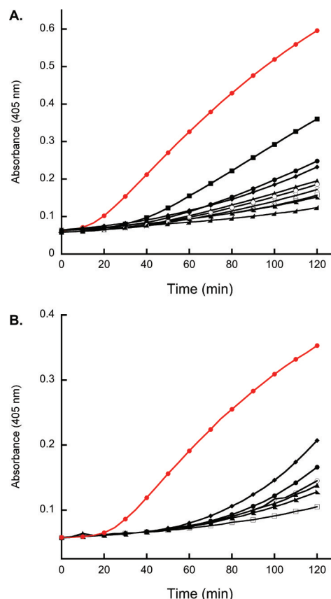
Figure 6. Representative plots from inner-membrane permeabilization assays. ONP formation monitored at 405 nm following incubation of E. coli ML35 with 2 μM of peptide and 2.5 mM ONPG at 37 °C (10 mM sodium phosphate buffer, 1% TSB, pH 7.4). (A) Comparison of HD5 ox with the Ser mutant peptides. (red ●) HD5 ox , (●) HD5[Ser 3,31 ] ox (5-20)(10-30), (left-tilting ▲) HD5[Ser 3,31 ] ox (5-30)(10-20), (◆) HD5[Ser 3,31 ] ox (5-10)(20-30), (▲) HD5[Ser 10,30 ] ox (3-20)(5-31), (■) HD5[Ser 5,20 ] ox (3-31)(10-30), (right-tilting ▲) HD5[Ser 5,20 ] ox (3-30)(10-31), (○) HD5[Ser 10,30 ] ox (3-31)(5-20), (×) HD5[Ser hexa ] ox . (B) Comparison of HD5 ox with the Ala mutant peptides. (red ●) HD5 ox , (●) HD5[Ala 3,31 ] ox (5-20)(10-30), (left-tilting ▲) HD5[Ala 3,31 ] ox (5-30)(10-20), (◆) HD5[Ala 3,31 ] ox (5-10)(20-30), (▲) HD5[Ala 10,30 ] ox (3-20)(5-31), (○) HD5[Ala 10,30 ] ox (3-31)(5-20). Results from inner-membrane permeabilization assays where E. coli ML35 were treated with varying concentrations of each peptide are available as Supporting Information.
