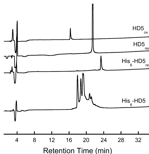
Figure 2. Representative analytical HPLC traces (220 nm absorption) of His 6 -HD5, purified HD5 red and purified HD5 ox (variable sample concentrations). TCEP was added to Ni-NTA purified His 6 -HD5 to provide the fully reduced sample His 6 -HD5 red (75 mM HEPES buffer, pH 7.4).
