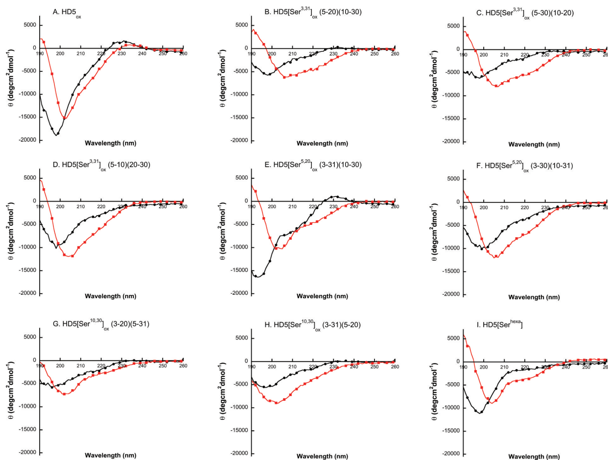
Figure 4. CD spectra of HD5 ox and the Ser mutant peptides in the absence (black ●) and presence (red ■) of 10 mM SDS (5 mM sodium phosphate buffer, pH 7.0). (A) HD5 ox . (B) HD5[Ser 3,31 ] ox (5-20)(10-30). (C) HD5[Ser 3,31 ] ox (5-30)(10-20). (D) HD5[Ser 3,31 ] ox (5-10)(20-30). (E) HD5[Ser 5,20 ] ox (3-31)(10-30). (F) HD5[Ser 5,20 ] ox (3-30)(10-31). (G) HD5[Ser 10,30 ] ox (3-20)(5-31). (H) HD5[Ser 10,30 ] ox (3-31)(5-20). (I) HD5[Ser hexa ] ox . CD spectra for the Ala mutants are available as Supporting Information.
